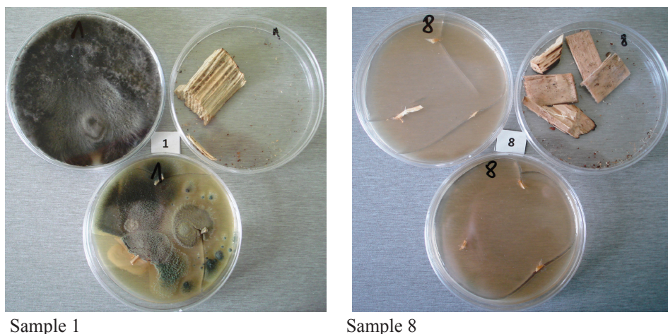
Fig. 3. Exemplary growth of filamentous fungi on a standard mineral-malt culture medium and the samples from which the inocula were taken
