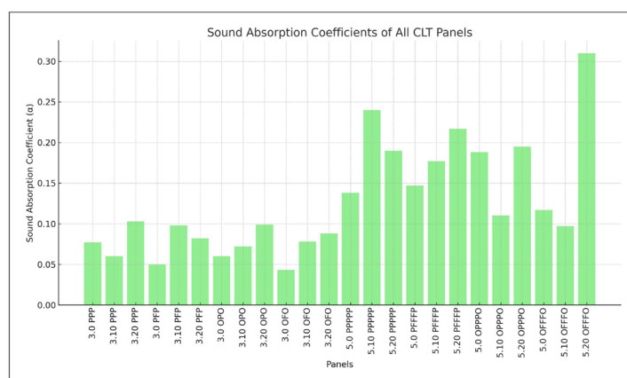
Fig. 12. Average values of sound absorption coefficients of three- and five-layer CLT panels
