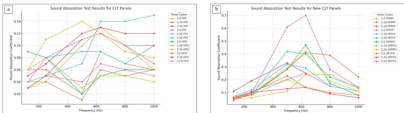
Fig. 11. Sound absorption test results for CLT panels: a) 3-layer CLT panels, b) 5-layer CLT panels
