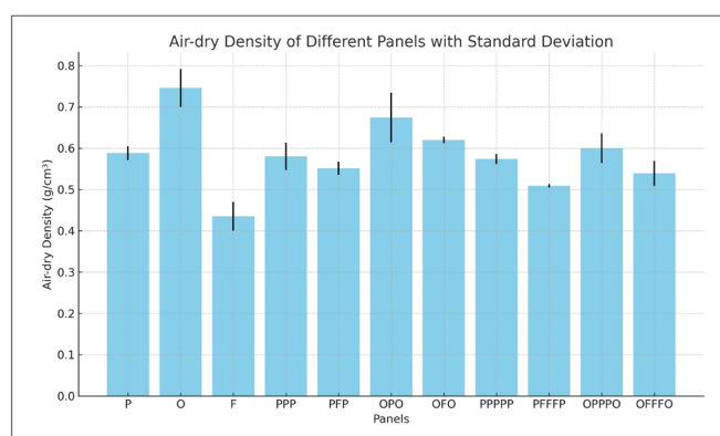
Fig. 7. Air-dry density values of CLTs
