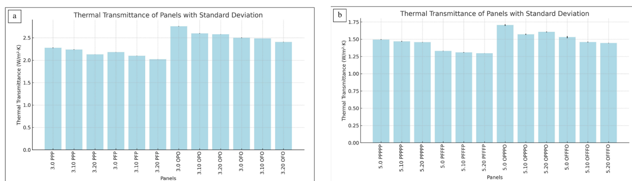
Fig. 10. Heat transmittance coefficient: a) three-layer CLT panels, b) five-layer CLT panels
