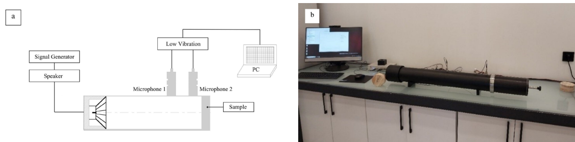
Fig. 6. a) Schematic diagram of the device used in the sound absorption test, b) impedance tube and test setup
