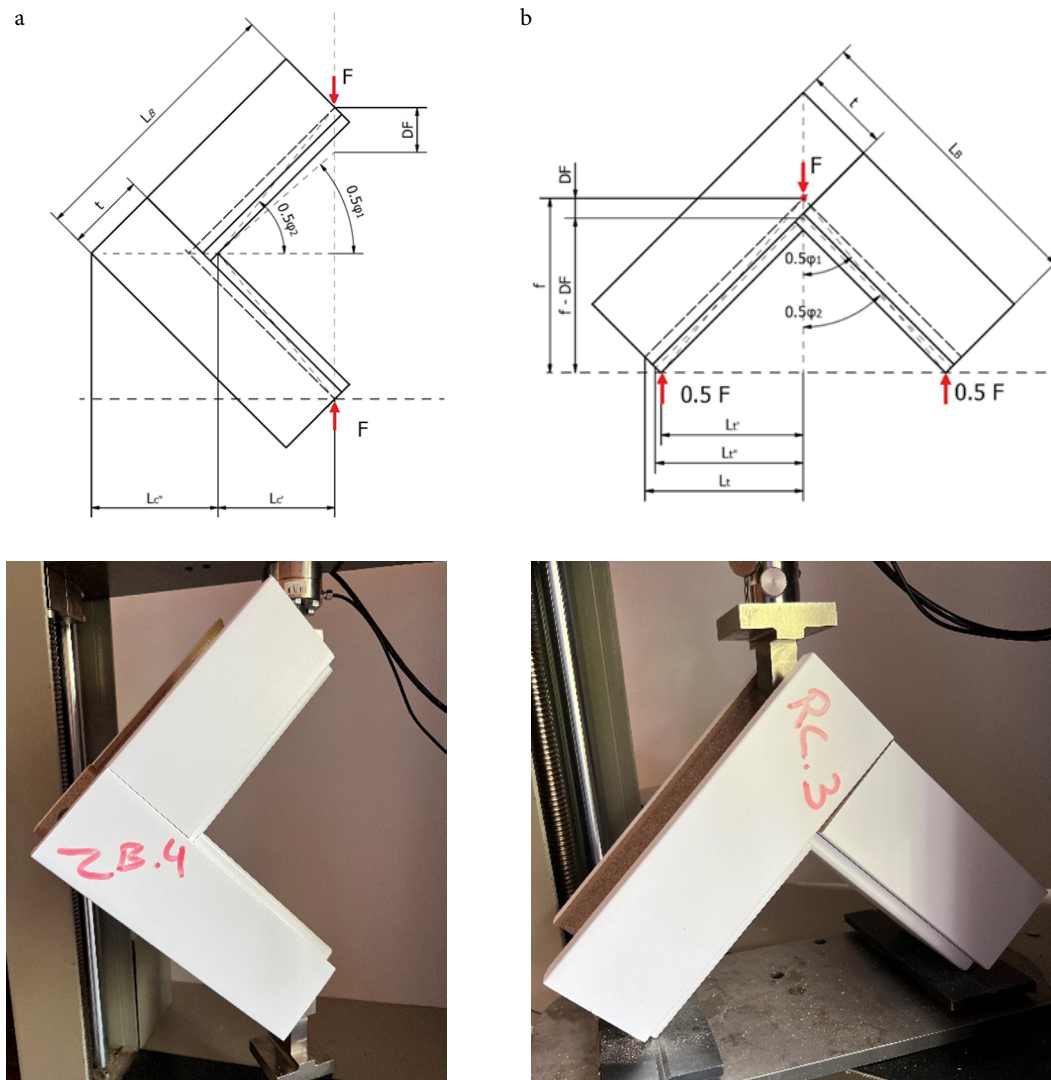
Fig. 1. Samples being tested on a testing machine: a) compression test, b) tension test
