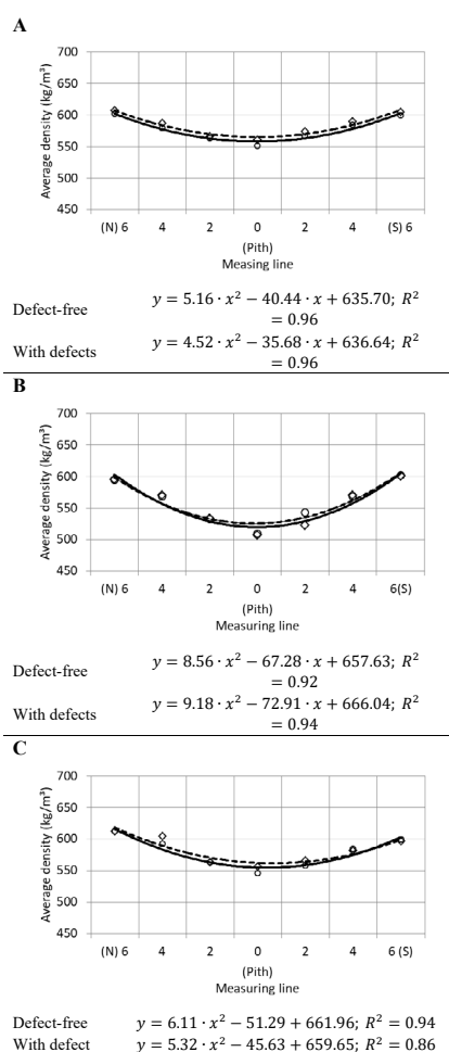
Fig. 2. Distribution of mean values of density on a transverse section of middle-sized silver birch timber: whole log (A), at breast height (B), at \frac{1}{4} log height (C)
