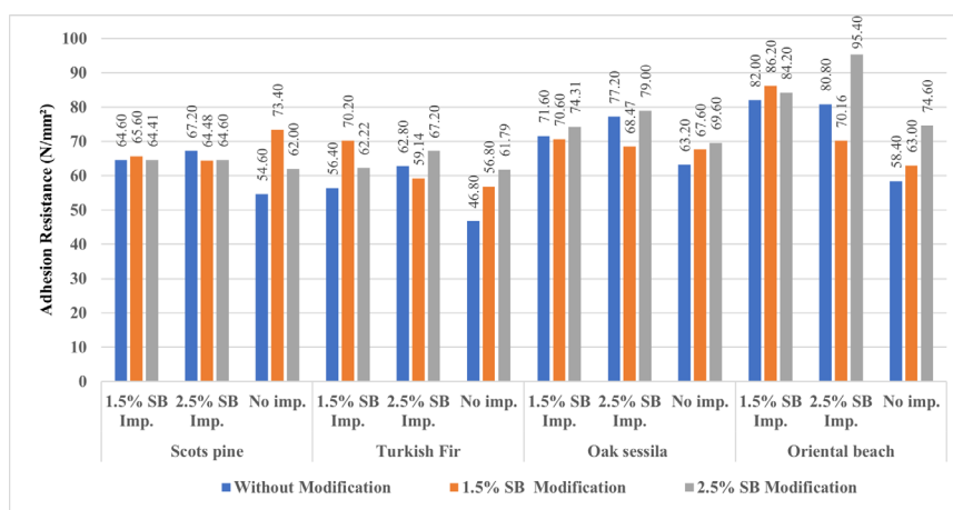
Fig. 8. Comparison of results depending on the interaction between wood species, impregnant concentration and varnish modification
