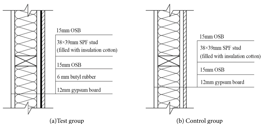
Fig. 3. Partition structure diagram
