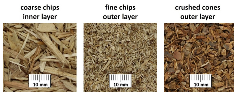
Fig. 1. View of wood chips and shredded pine cones used in the production of the panel
