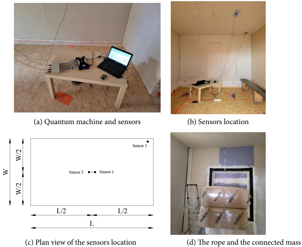
Fig. 4. Measurement system
