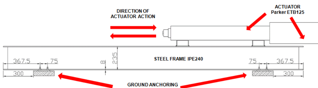
Fig. 1. Sketch of the experimental setup – side view (mm)
