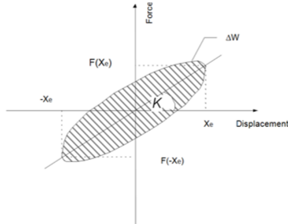
Fig. 8. Hysteresis loop
