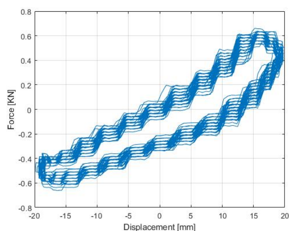
Fig. 12. Hysteresis loops for the screwed wooden frame – 3 Hz and 20 mm
